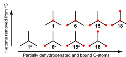
Figure 1. Forms of partially dehydrogenated isobutane intermediates organized by the total number of partially dehydrogenated C atoms and the number of H atoms (0 or 1) removed from the central ^3C . Dots indicate an attachment position where a C atom has lost one or more H atoms, and binds to the metal surface. Numbers near each structure indicate the number of different C–C cleavage transition states formed from intermediates with those surface attachments. a C–C cleavage within molecular isobutane not calculated. b Only C–C cleavage of partially dehydrogenated C–C bonds (indicated by dashed lines) was calculated.
