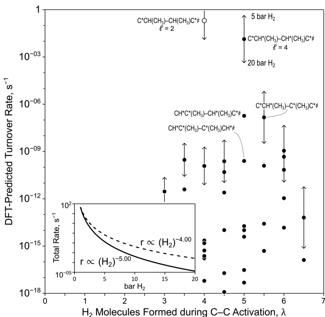
Figure 13. DFT-predicted hydrogenolysis rates ( \text{s}^{-1} ) for 2,3-dimethylbutane (10 kPa) cleavage via transition states shown in Figure 9 at 10 bar \text{H}_2 , up/down arrows represent 5 and 20 bar \text{H}_2 , respectively (the size of the bars depend only on \lambda , so they are omitted from most points for clarity). C–C cleavage of \text{C}^*\text{CH}(\text{CH}_3)\text{CH}(\text{CH}_3)\text{C}^* shown with a two-site ( l = 2 , open symbol) and four-site ( l = 4 ) transition state. (Inset) Total rate from 1 to 20 bar \text{H}_2 , showing a DFT-predicted \lambda value of 5.00 when l = 4 for \text{C}^*\text{CH}^*(\text{CH}_3)-\text{CH}^*(\text{CH}_3)\text{C}^*\ddagger or a \lambda of 4.00 when l = 2 for \text{C}^*\text{CH}(\text{CH}_3)-\text{CH}(\text{CH}_3)\text{C}^*\ddagger (dashed line).
