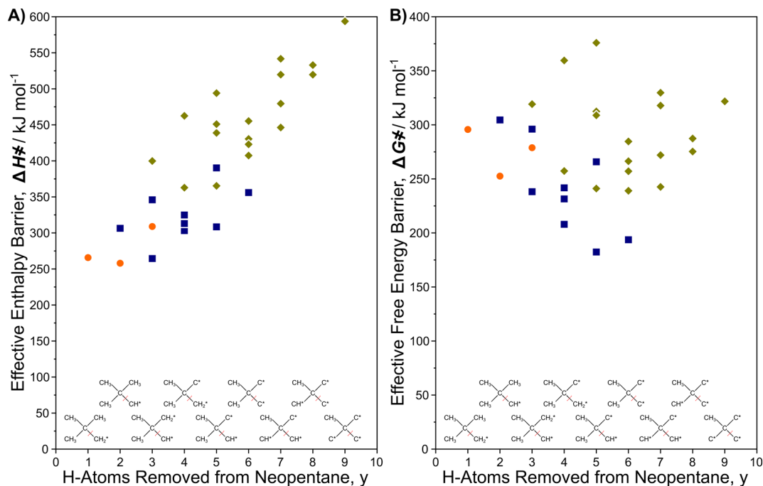
Figure 6. (A) \Delta H^\ddagger and (B) \Delta G^\ddagger for C–C bond activations of neopentane-derived intermediates via C–C activations of: \alpha -bound intermediates ( \bullet , orange); \alpha,\gamma -bound intermediates ( \blacksquare , blue); \alpha,\gamma,\delta -bound intermediates ( \blacklozenge , brown). The intermediate with the lowest \Delta H^\ddagger and \Delta G^\ddagger is shown near the ordinate for each number of H atoms removed from neopentane. Tables S2, S3, and S6 in the SI show y , I , \lambda , \Delta H_{\text{act}} , \Delta H^\ddagger , \Delta S^\ddagger , and \Delta G^\ddagger for all transition states shown above. Color version (to add contrast between symbols) available online.
