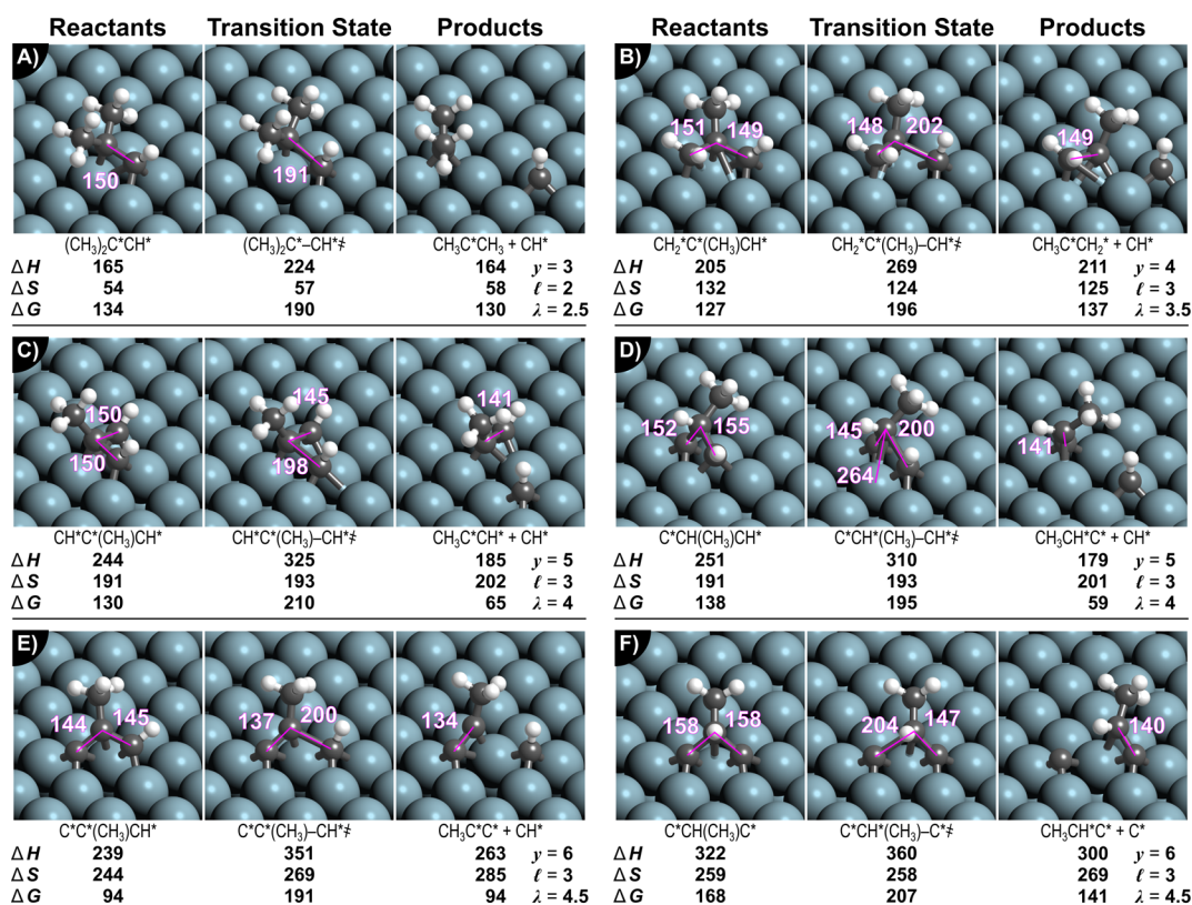
Figure 3. Reactant, product, and transition state structures for C–C cleavage of isobutane via (A) (\text{CH}_3)_2\text{C}^*\text{CH}^*\ddagger , (B) \text{CH}_2^*\text{C}^*(\text{CH}_3)\text{CH}^*\ddagger , (C) \text{CH}^*\text{C}^*(\text{CH}_3)\text{CH}^*\ddagger , (D) \text{C}^*\text{CH}(\text{CH}_3)\text{CH}^*\ddagger , (E) \text{C}^*\text{C}^*(\text{CH}_3)\text{CH}^*\ddagger , and (F) \text{C}^*\text{CH}(\text{CH}_3)\text{C}^*\ddagger . Enthalpies ( \Delta H , kJ mol −1 ), entropies ( \Delta S , J mol −1 K −1 ) and free energies ( \Delta G , kJ mol −1 ) for forming each state (and stoichiometric amounts of H 2 ) from isobutane and a H*–covered surface are shown. Notable C–C bond distances shown in pm.
