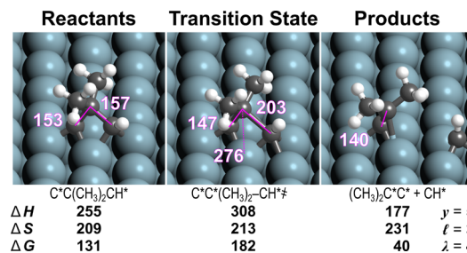
Figure 7. Reactant, product and transition state structures for C–C cleavage of neopentane via \text{C}^*(\text{CH}_3)_2-\text{CH}^* . Enthalpies ( \text{kJ mol}^{-1} ), entropies ( \text{J mol}^{-1} \text{K}^{-1} ) and free energies ( \text{kJ mol}^{-1} ) for forming each state (and stoichiometric amounts of \text{H}_2 ) from neopentane and a \text{H}^* -covered surface are shown. Notable C–C bond distances shown in pm.
